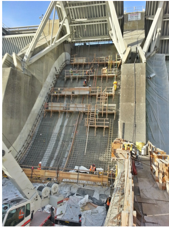
Figure 5 Priest Rapids Fish Bypass, Bay 20 Apron and Ogee Concrete Curing and Preparation Work. December 2013.
