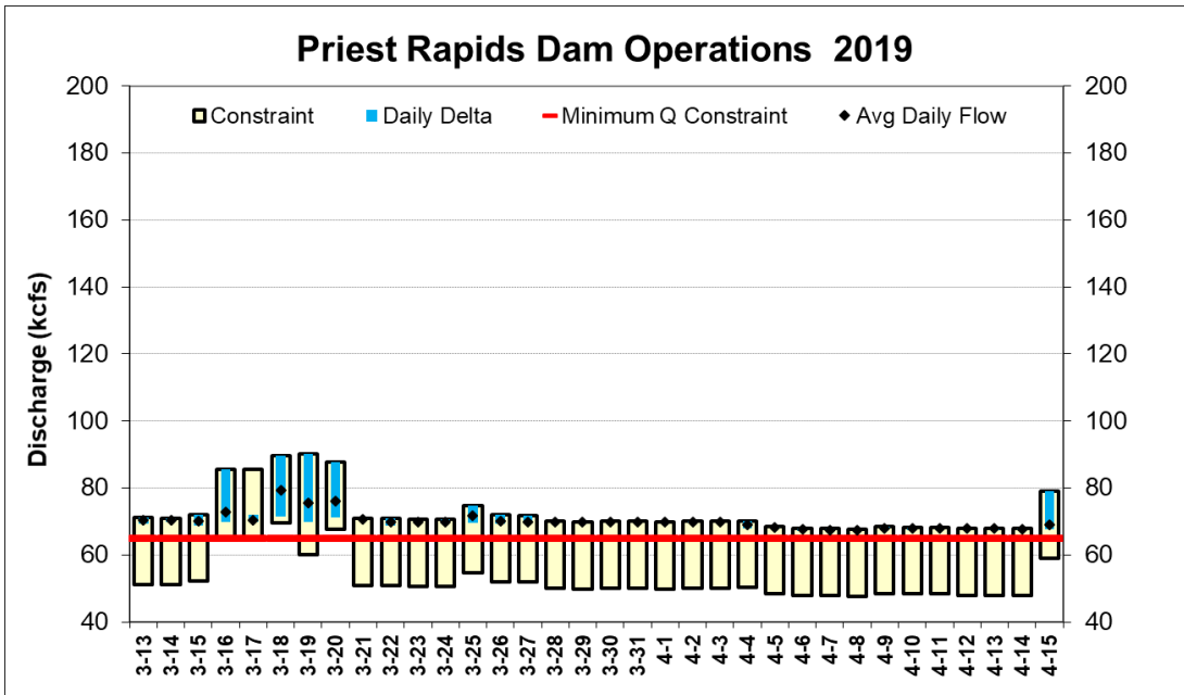
Figure 14 Mean, minimum, maximum hourly discharge and daily fluctuation from Priest Rapids Dam, March 13 – April 15, 2019.
