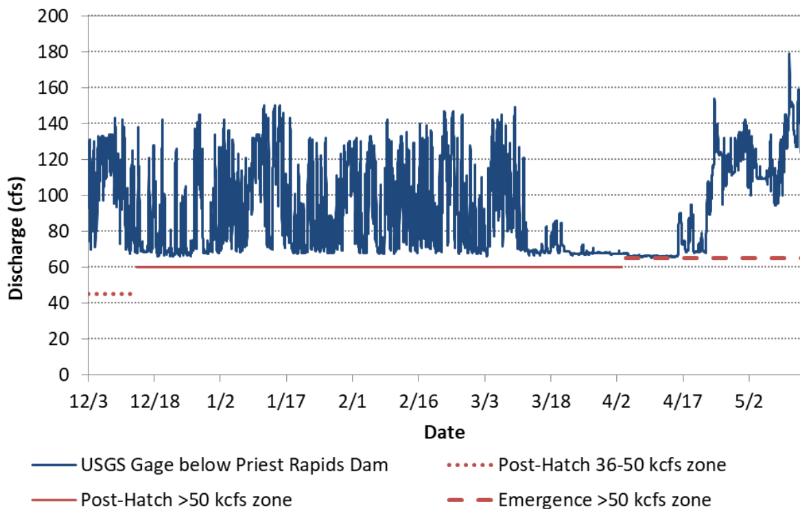
Figure 10 Discharge during the 2018-2019 Post Hatch and Emergence Periods measured at USGS Gage 12472800 below Priest Rapids Dam and the Protection Level Flow.
