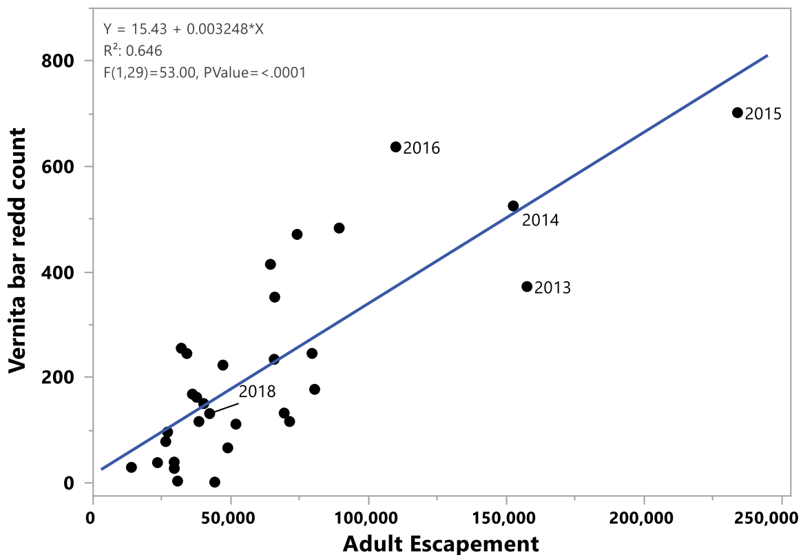
Figure 4 Relationship between Hanford Reach adult escapement and redds above the 50 kcfs elevation observed during the Vernita Bar spawning surveys (1988-2018).
