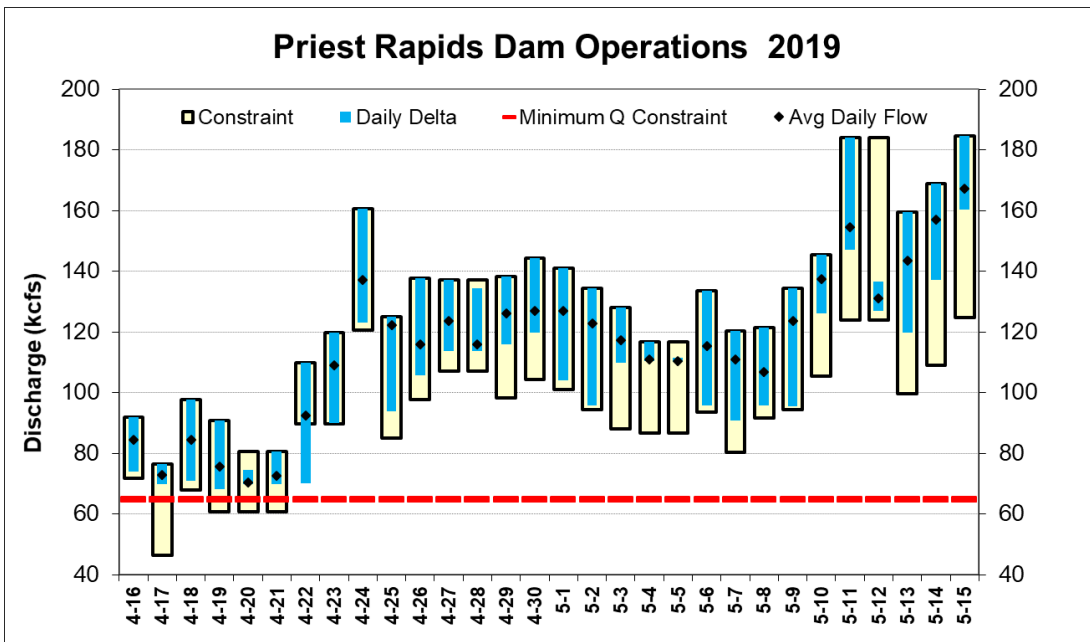
Figure 15 Mean, minimum, maximum hourly discharge and daily fluctuation from Priest Rapids Dam, April 16 – May 15, 2019.
