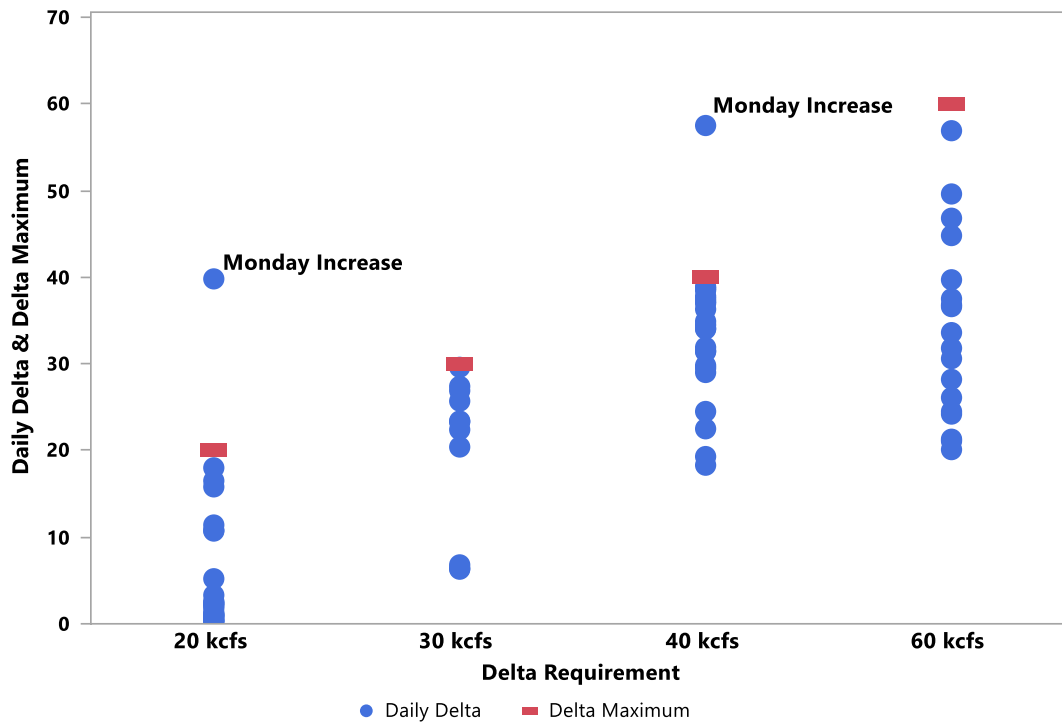
Figure 13 Summary of 2019 Priest Rapids Dam daily discharge deltas and delta maximum by constraint category.
