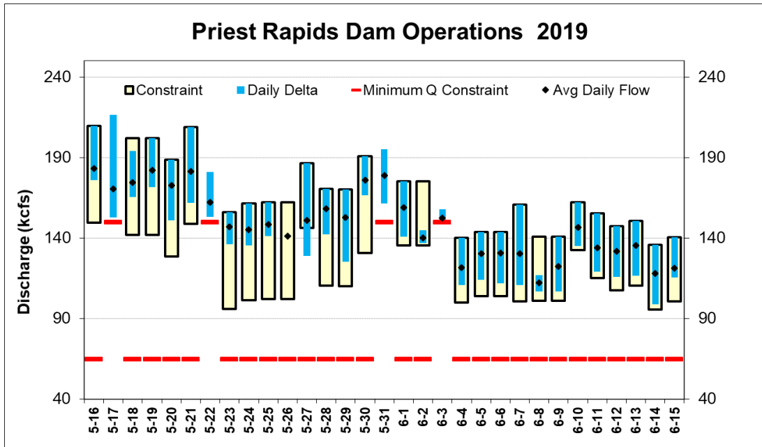
Figure 16 Mean, minimum, maximum hourly discharge and daily fluctuation from Priest Rapids Dam, May 16 – June 15, 2019.
