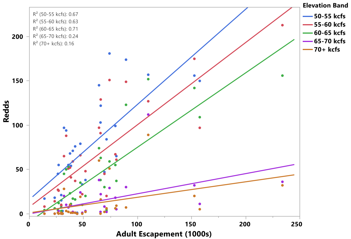
Figure 5 Relationship between Hanford Reach escapement and redd counts on Vernita Bar by kcfs elevation bands (1988-2018).
