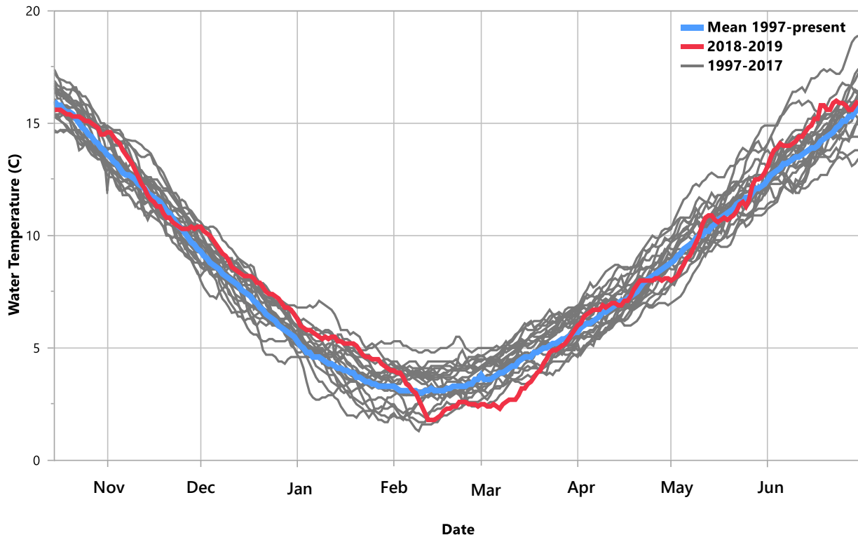
Figure 7 Daily river temperatures on the Hanford Reach of the Columbia River during the protection season for brood years 1997-2017 (grey lines), the 2018 brood year (red line), and the daily mean temperature for brood years 1997-2018 (blue line).
