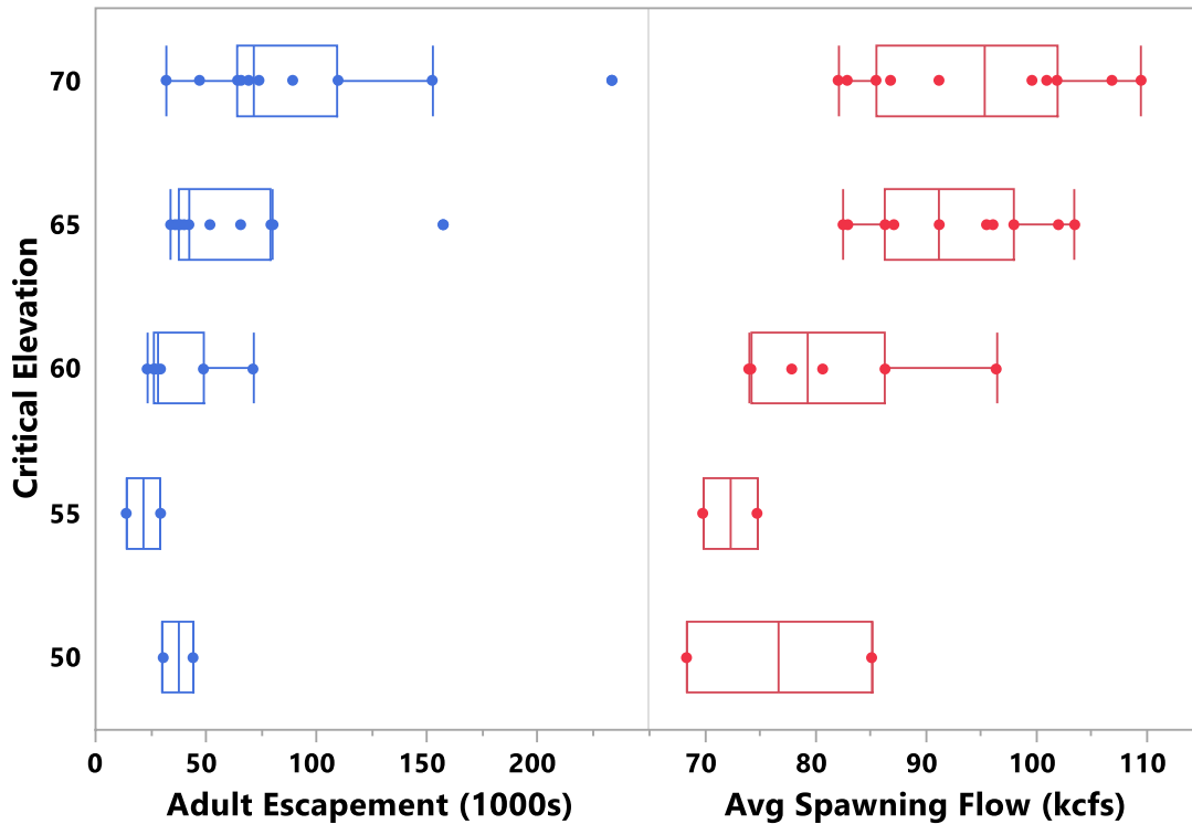
Figure 6 Relationship between Hanford Reach adult escapement and the Critical Elevation (left) and Priest Rapids Dam average discharge during peak spawning and Critical Elevation (right) (1988-2018).
