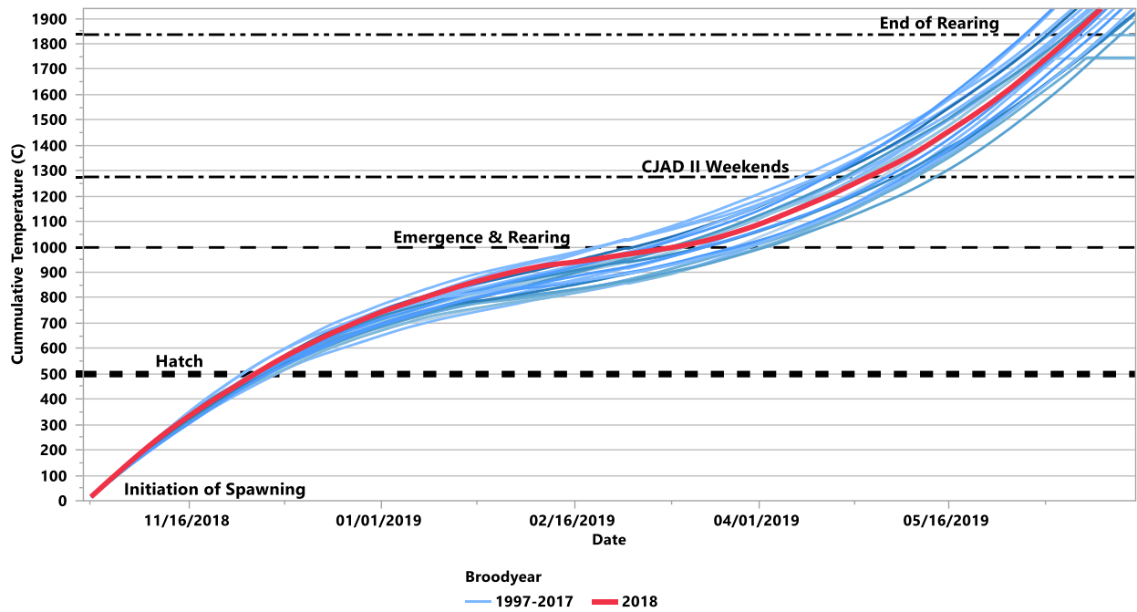
Figure 8 The accumulation of temperature units in the Hanford Reach and Protection Periods during the protection season for brood years 1997-2017 (blue lines) and brood year 2018 (red line).
