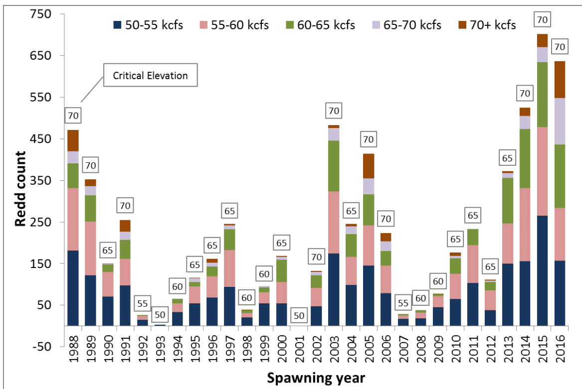
Figure 3 Final redd abundance and distribution from ground surveys on Vernita Bar, 1988-2016. Final redd counts are not consistently conducted in the 36-50 kcfs zone and are not included in this figure. The Critical Elevation for each year is listed above the bars.
