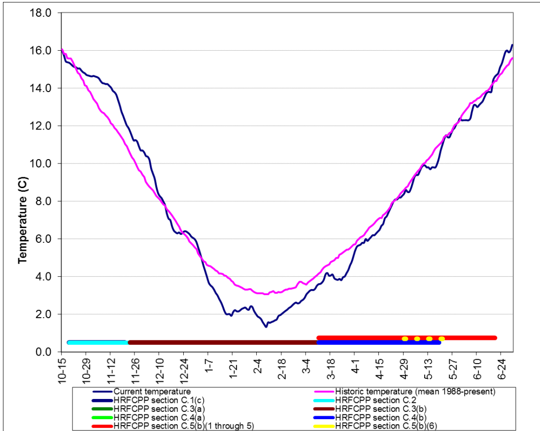
Figure 7 Mean daily river temperatures on the Hanford Reach of the Columbia River and estimated timing of fall Chinook salmon protections based on accumulated temperature units (ATU), 2016-17.
