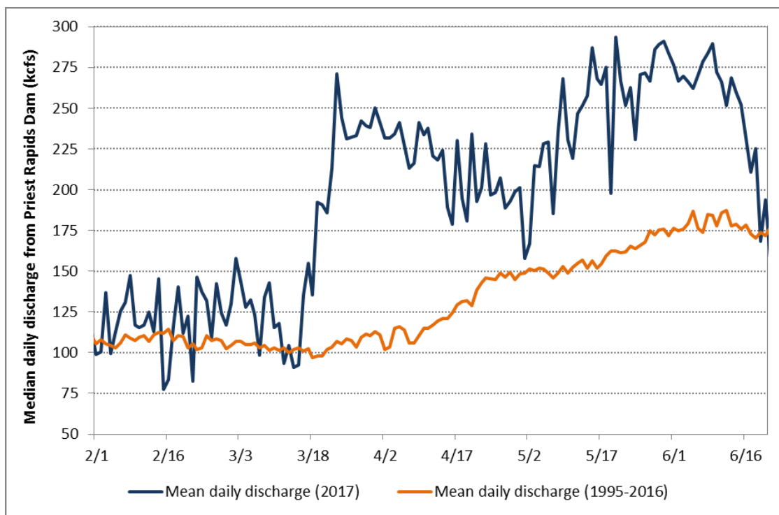
Figure 10 Mean daily discharge from Priest Rapids Dam during the Emergence and Rearing Periods in 2017 and the mean from 1995-2016 under the VBSA and HRF CPPA.
