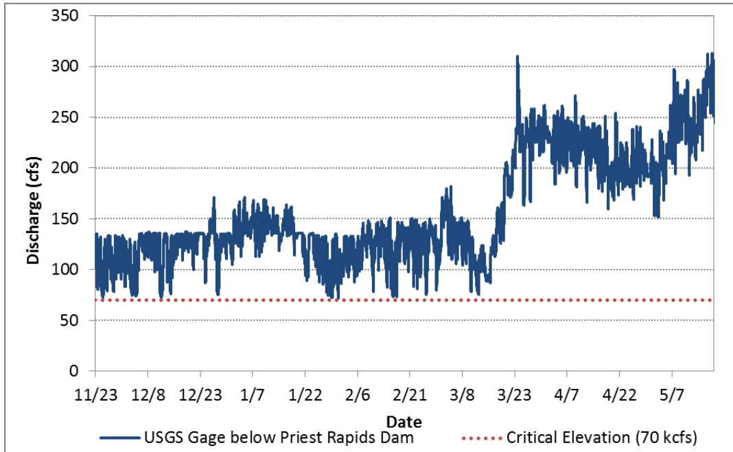
Figure 12 Discharge during the 2015-2016 Post Hatch and Emergence and Rearing periods measured at USGS Gage 12472800 below Priest Rapids Dam with the Critical Elevation (70 kcfs, dotted line).
