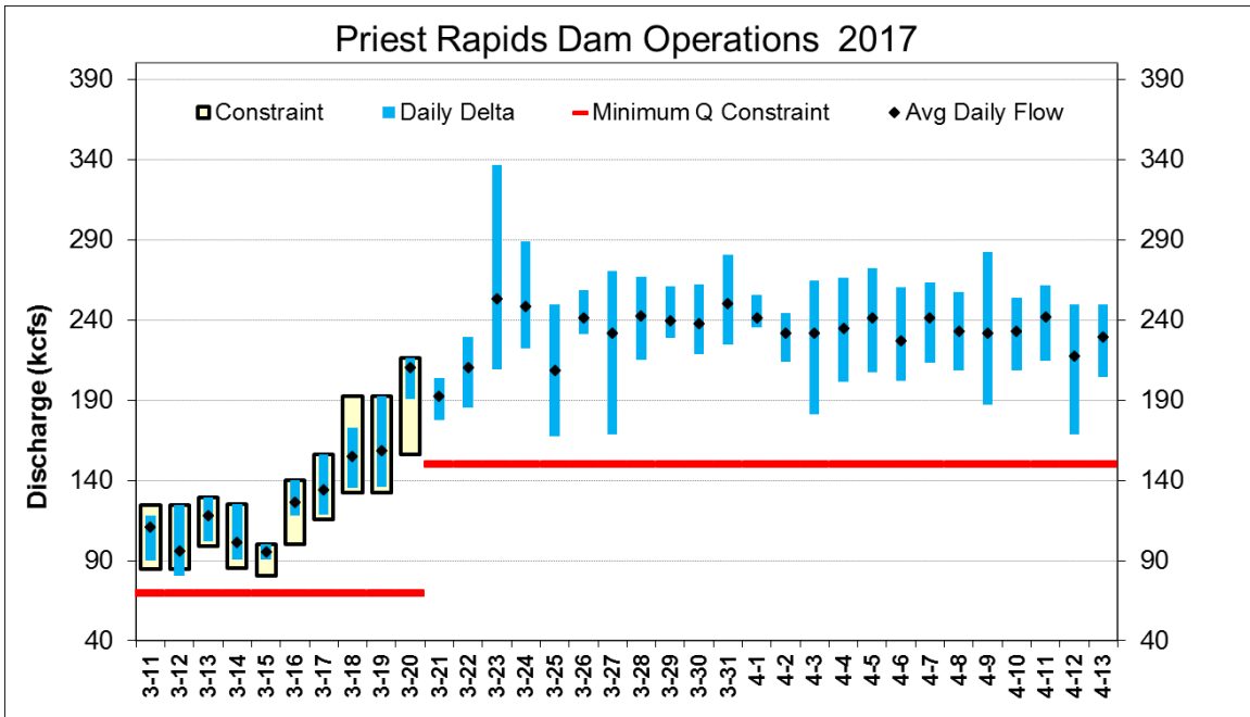
Figure 14 Mean, minimum, maximum hourly discharge and daily fluctuation from Priest Rapids Dam, March 11 – April 13, 2017.
