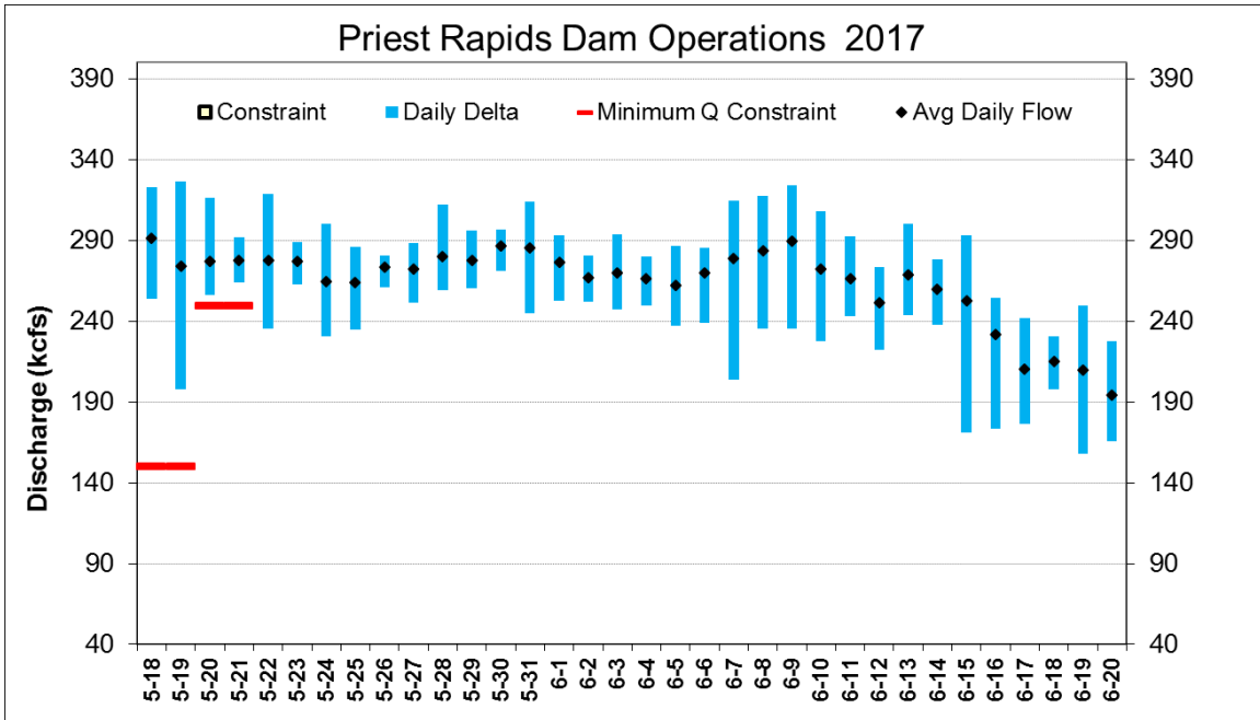
Figure 16 Mean, minimum, maximum hourly discharge and daily fluctuation from Priest Rapids Dam, May 18 – June 20, 2017.
