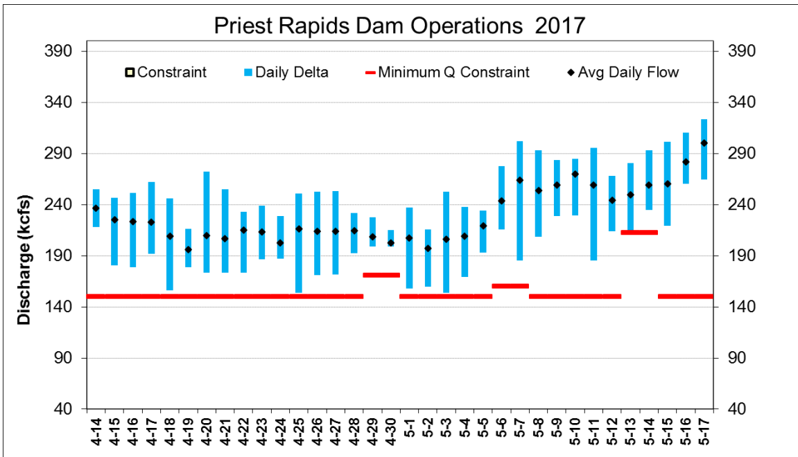
Figure 15 Mean, minimum, maximum hourly discharge and daily fluctuation from Priest Rapids Dam, April 14 – May 17, 2017.
