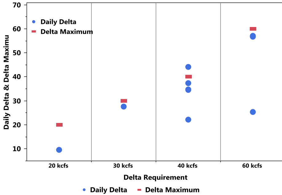
Figure 13 Summary of 2017 Priest Rapids Dam daily discharge deltas and delta maximum by constraint category.
