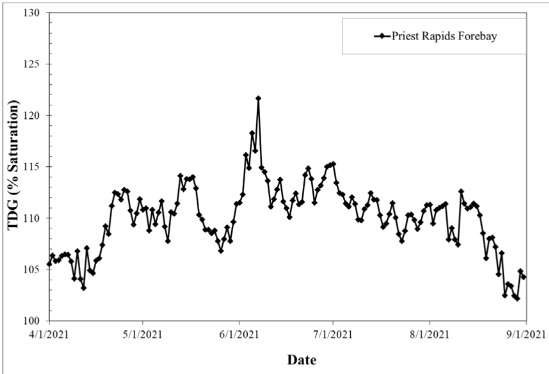
Figure 8 Total dissolved gas values (average of the 12-highest hourly TDG values in a day) from the 2021 fish-spill season recorded at the Priest Rapids Dam forebay FSM station. Priest Rapids Project, mid-Columbia River, WA.
