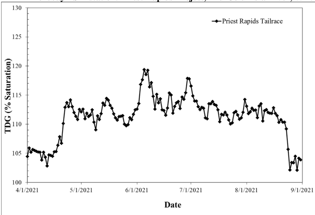
Figure 9 Total dissolved gas values (average of the 12-highest hourly TDG values in a day) from the 2021 fish-spill season recorded at the Priest Rapids Dam tailrace FSM station. Priest Rapids Project, mid-Columbia River, WA.
