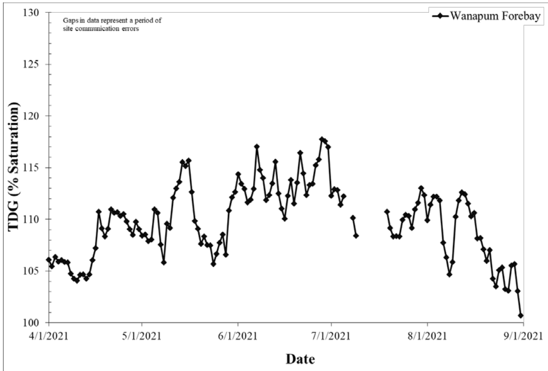
Figure 6 Total dissolved gas values (average of the 12-highest hourly TDG values in a day) from the 2021 fish-spill season recorded at the Wanapum Dam forebay FSM station. Priest Rapids Project, mid-Columbia River, WA.
