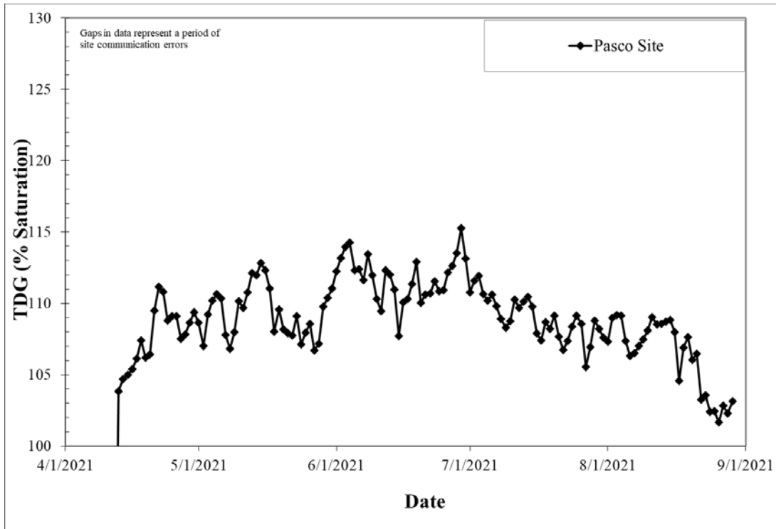
Figure 10 Total dissolved gas values (average of the 12-highest hourly TDG values in a day) from the 2021 fish-spill season recorded at the Pasco FSM station, mid-Columbia River, WA.
