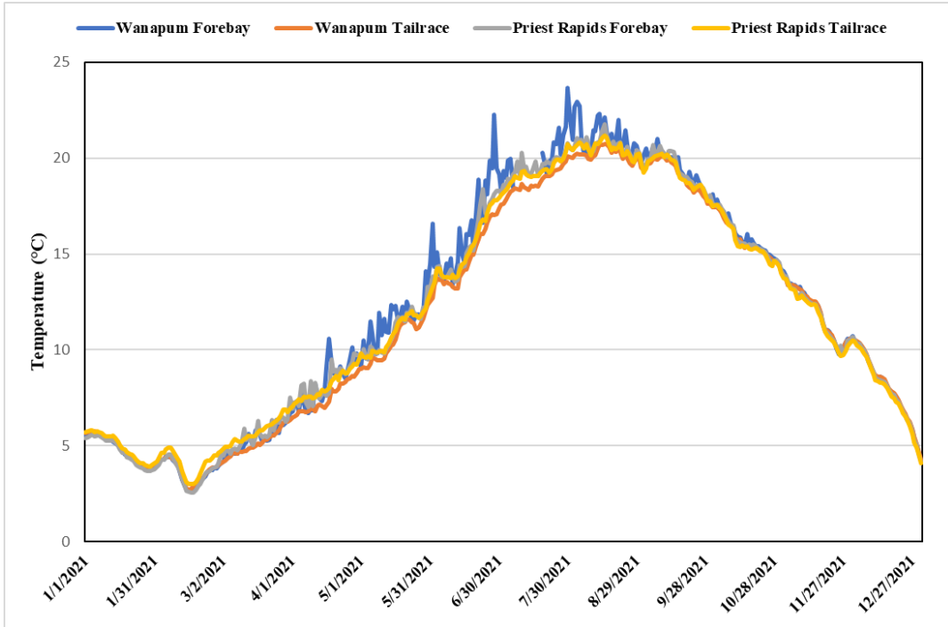
Figure 11 Daily maximum (1-DMax) water temperature values recorded at each fixed-site monitoring station (FSM station) in 2021, Priest Rapids Hydroelectric Project, mid-Columbia River, WA.
