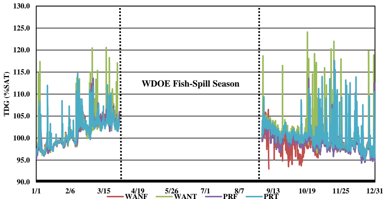
Figure 5 Hourly total dissolved gas values from the 2021 non-fish spill season, Priest Rapids Hydroelectric Project, mid-Columbia River, WA.
