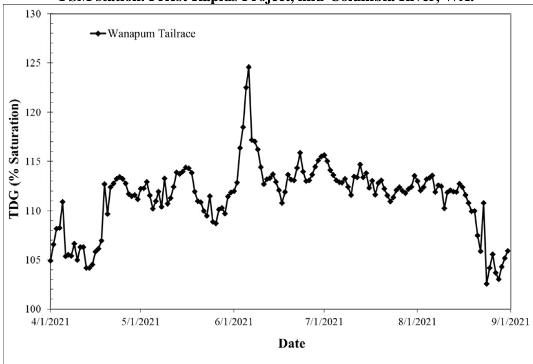
Figure 7 Total dissolved gas values (average of the 12-highest hourly TDG values in a day) from the 2021 fish-spill season recorded at the Wanapum Dam tailrace FSM station. Priest Rapids Project, mid-Columbia River, WA.
