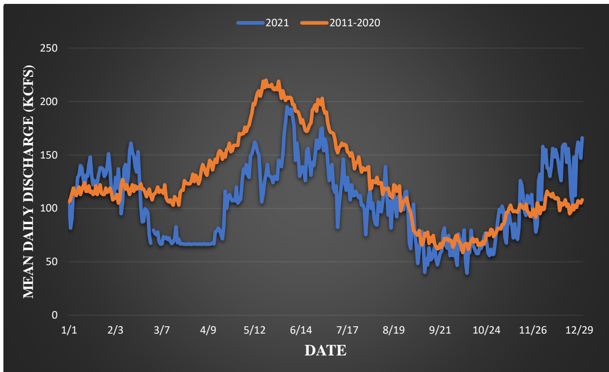
Figure 4 Comparison of 2021 vs. previous 10-year average of mean daily discharge values measured at the U.S. Geological Survey (USGS) streamflow gage #12472800 located 2.6 river miles below Priest Rapids Dam, Priest Rapids Hydroelectric Project, mid-Columbia River, WA.
